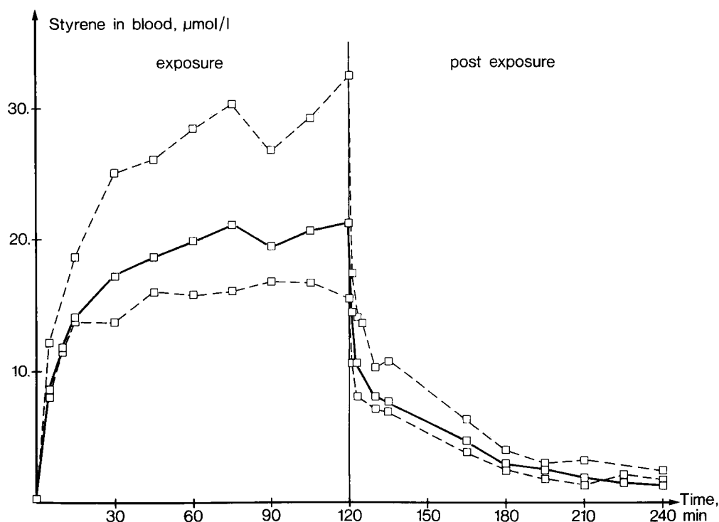
Fig. 2. The concentration of styrene in the arterial blood of seven subjects ( \square ) during and after exposure to a styrene concentration of about 2.88 \text{ mmol/m}^3 ( 300 \text{ mg/m}^3 ) for 2 h during physical exercise with a work load of 50 W. The solid line represents the mean value ( N = 7 ), and the two broken lines show the two subjects with the overall highest and lowest blood concentration.
