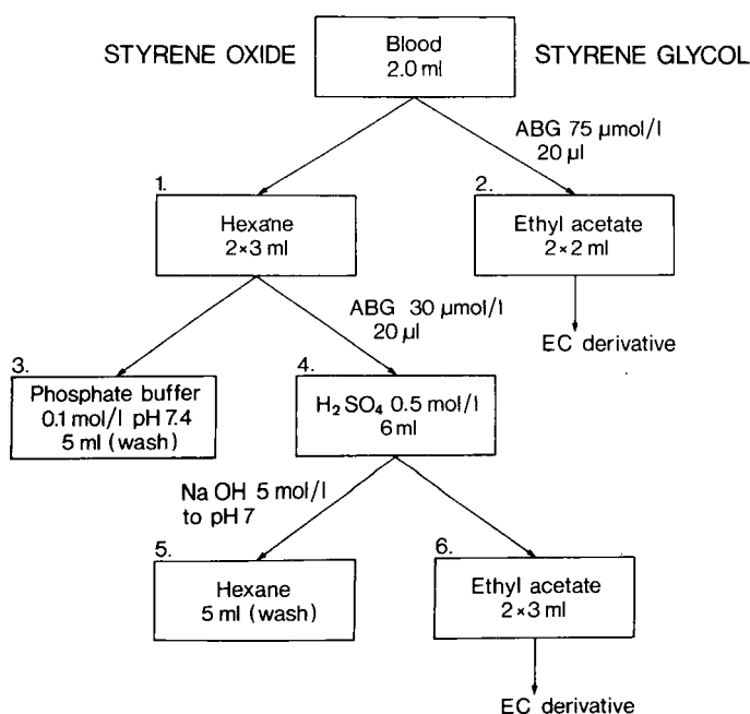
Fig 1. A scheme for the extraction of styrene oxide and styrene glycol from blood. Allylbenzene glycol (ABG) was added as the internal standard. The ethyl acetate extracts were treated with pentafluorobenzoyl chloride to make derivatives suitable for electron capture (EC) detection. (H 2 SO 4 = sulfuric acid, NaOH = sodium hydroxide)
