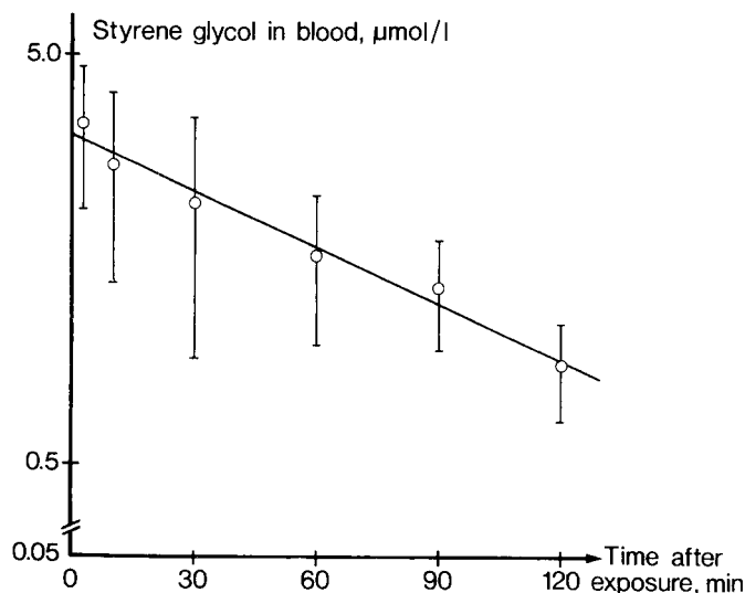
Fig 5. Semilogarithmic plot of the mean ( \pm SD) concentration of styrene glycol in the arterial blood after the end of exposure to a styrene concentration of about 2.88 mmol/m 3 (300 mg/m 3 ) for 2 h during physical exercise with a work load of 50 W. Individual regression lines were used to calculate the mean half-time of 72.1 (SD 13.3) min.
