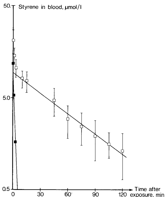
Fig 3. Semilogarithmic plot of the mean concentration ( \pm SD) of styrene in the arterial blood of seven subjects ( \square ) after the end of exposure to a styrene concentration of about 2.88 \text{ mmol/m}^3 ( 300 \text{ mg/m}^3 ) for 2 h during physical exercise with a work load of 50 W. The method of residuals was used to resolve the curve into a linear terminal phase and a linear initial phase ( \blacksquare ). Individual regression lines were used to calculate the mean half-time of the initial and terminal phase, 1.9 (SD 0.8) and 40.8 (SD 7.0) min, respectively.
