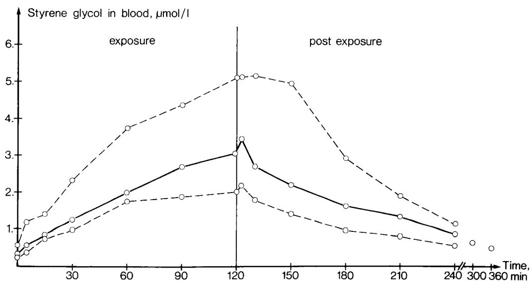
Fig 4. The concentration of styrene glycol in the arterial blood of seven subjects during and after exposure to a styrene concentration of about 2.88 \text{ mmol/m}^3 ( 300 \text{ mg/m}^3 ) for 2 h during physical exercise with a work load of 50 W. The solid line represents the mean value ( N = 7 ), and the two broken lines show the two subjects with the overall highest and lowest blood concentration. The mean concentration of styrene glycol in the venous blood is shown at 300 and 360 min.
