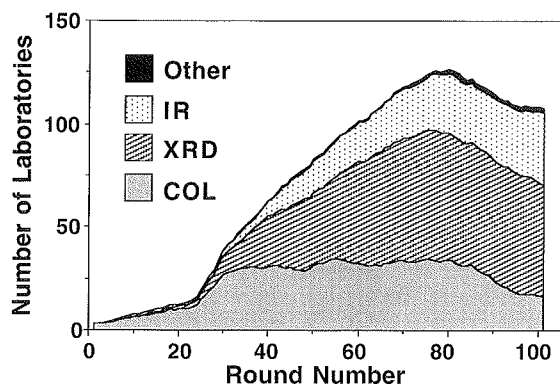
Figure 1. Cumulative number of laboratories using a particular method of silica analysis in the proficiency analytical testing (PAT) program. (IR = infrared spectroscopy, XRD = X-ray diffraction, COL = colorimetry)
